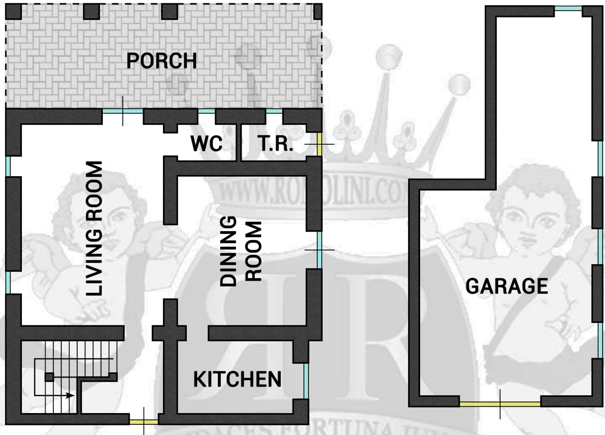
GROUND FLOOR
