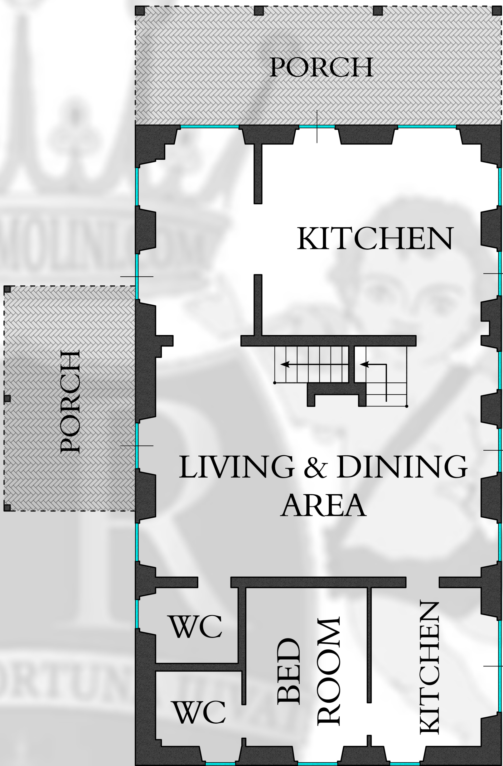
GROUND FLOOR
