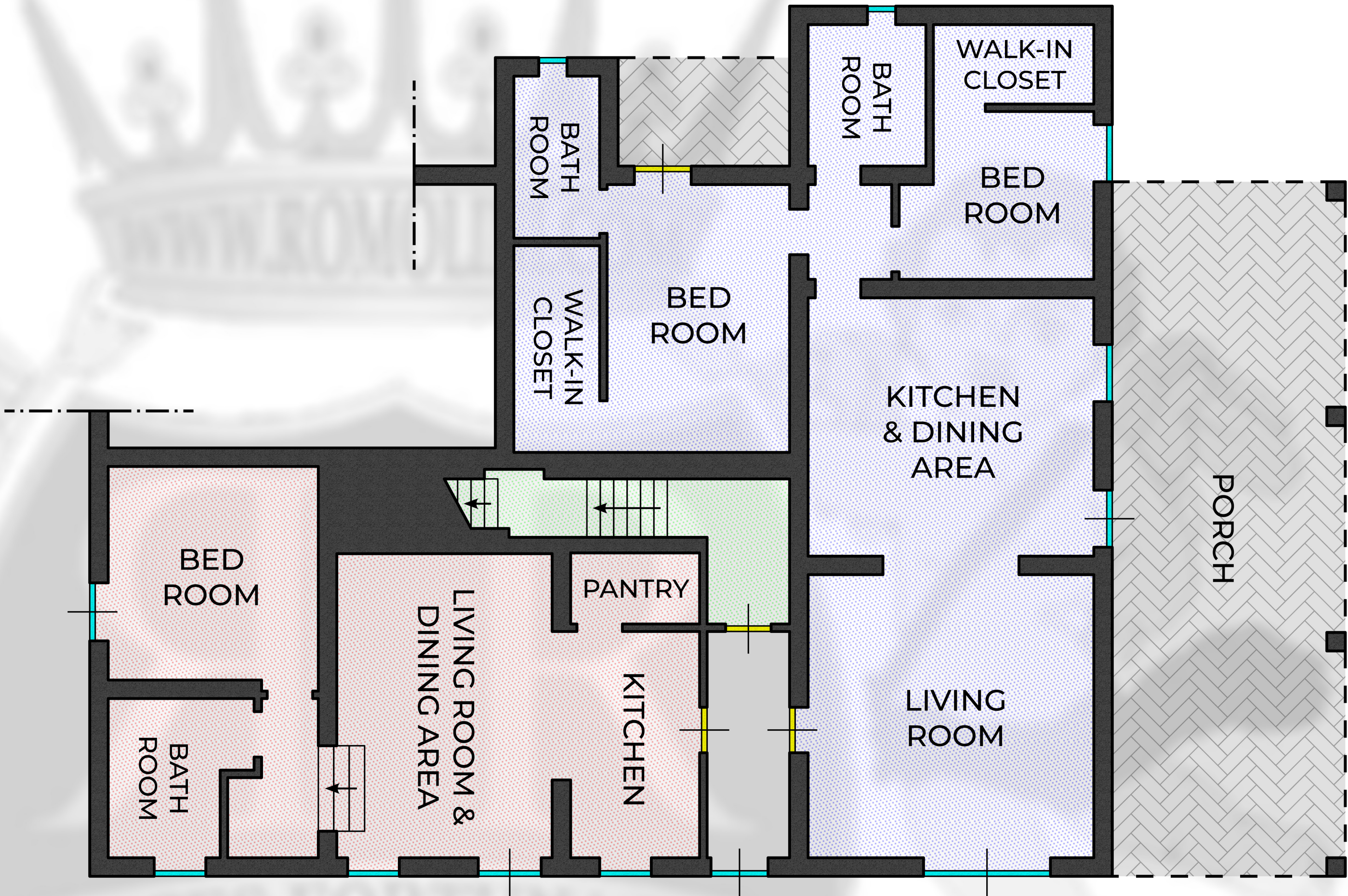
GROUND FLOOR
