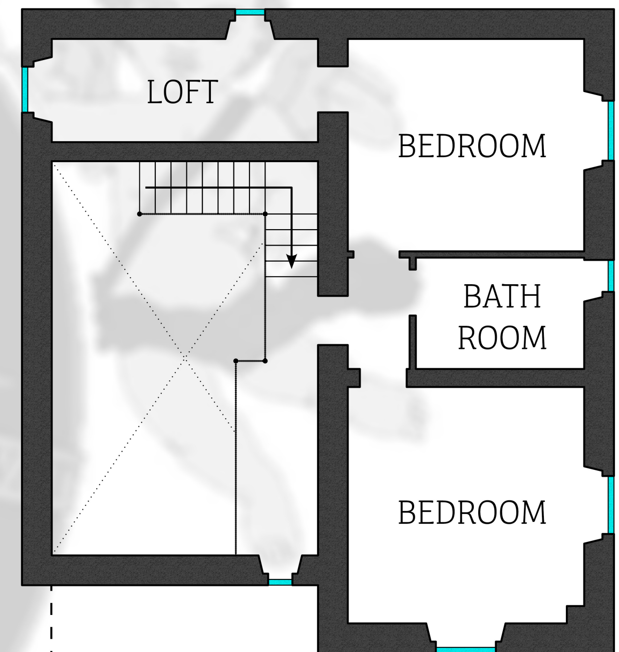
FIRST FLOOR
