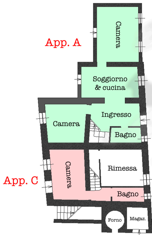
PIANO TERRA
